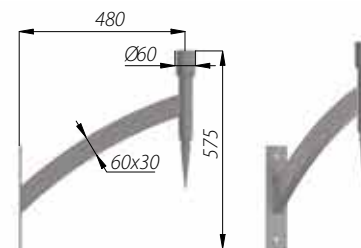
KA-D1 code: 478103/C... luminarias: OP, OPA-1, OS-1, OS-1 LED, OS-11 LED
