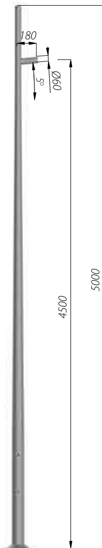
SAL-DL6 code: 42998/C...
