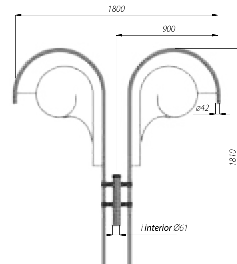
WA-20/2 code: 471202/C... luminarias: OW LED, DROP LED, OW
