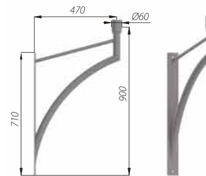
KA-A1 code: 478100/C... luminarias: OP, OPA-1, OS-1, OS-1 LED, OS-11 LED
