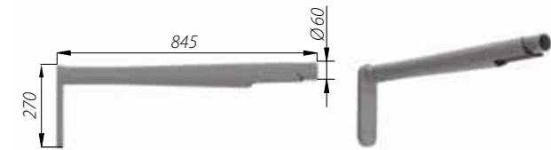
KA-10 code: 478220/C.../C... luminaria ISKRA LED
