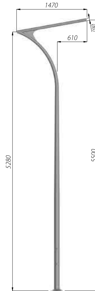
SAL DS-52 code: 42225/C...
