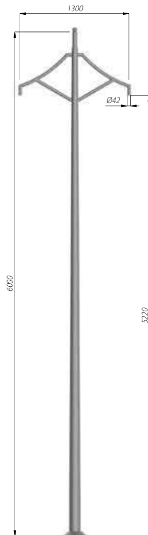
SAL-M2 code: 42309/C...
