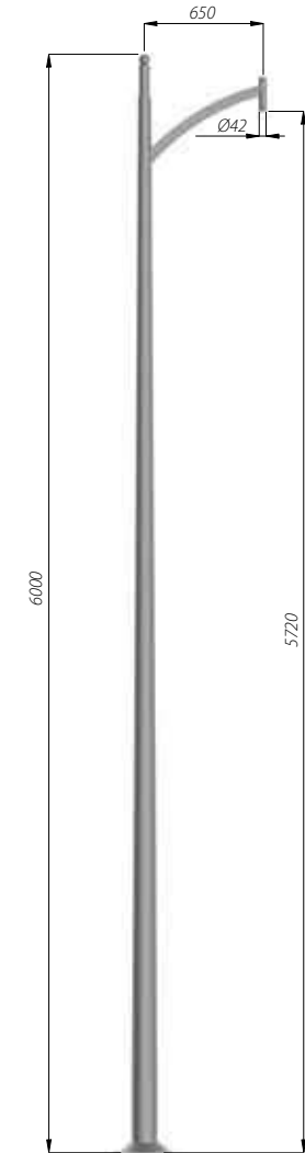
SAL-K1 code: 42330/C...
