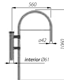
WA-14/1 code: 471141/C... luminarias: OW LED, DROP LED, OW
