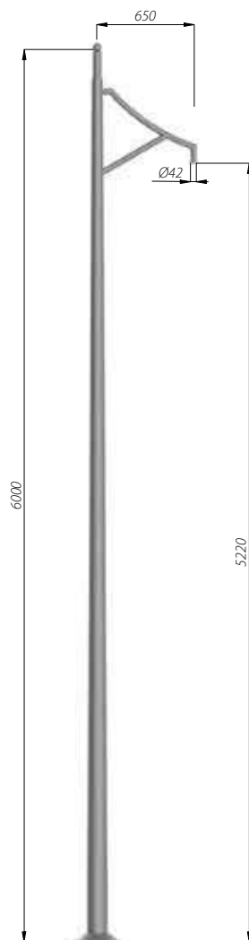
SAL-M1 code: 42308/C...
