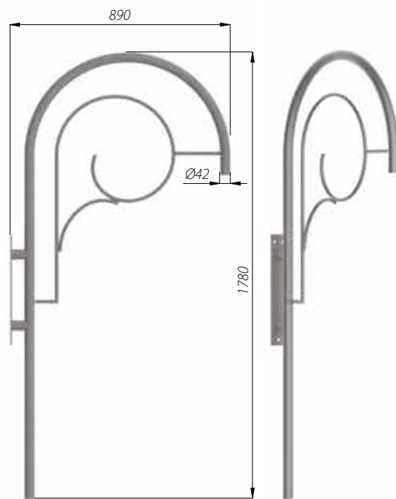
KA-20 code: 478200/C... luminarias: OW LED, DROP LED, OW
