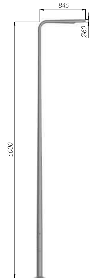
SAL DL-10 code: 42999/C.../C... Luminaria ISKRA LED
