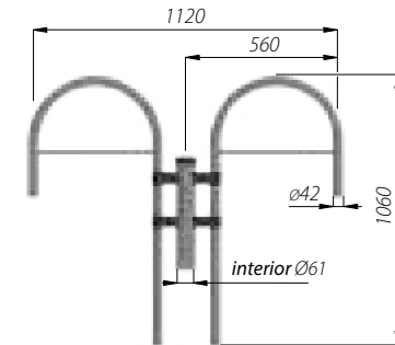
WA-14/2 code: 471142/C... luminarias: OW LED, DROP LED, OW
