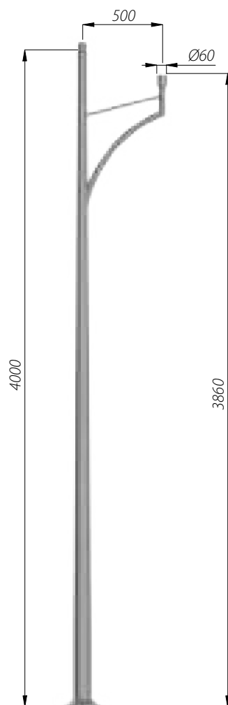
SAL-A1. code: 42209/C...
