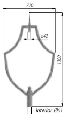
WA-4 code: 471040/C... luminarias: OW LED, OW
