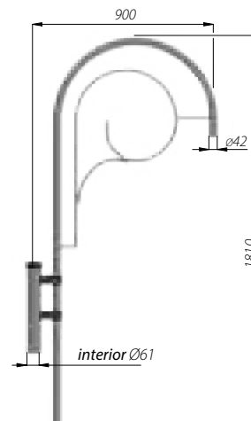
WA-20/1 code: 471201/C... luminarias: OW LED, DROP LED, OW
