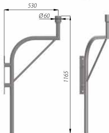
KA-5 code: 478050/C... luminarias: OP, OPA-1
