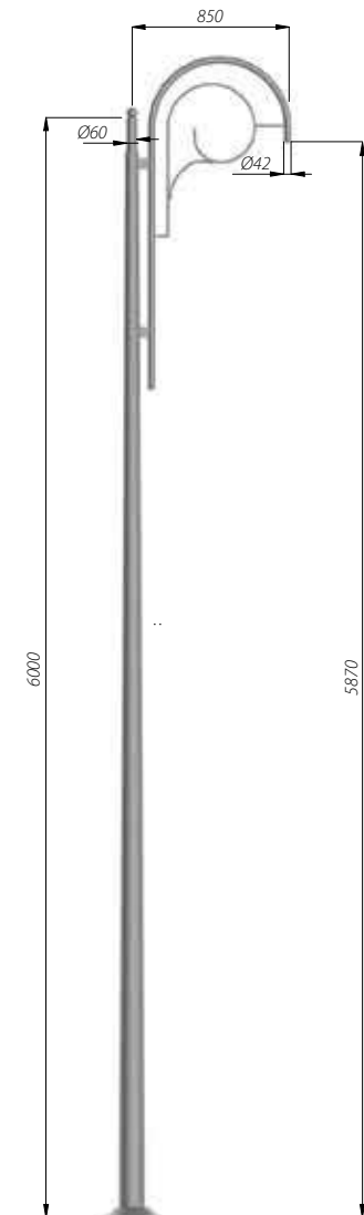
SAL-R1 code: 42334/C...
