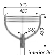
WA-1 code: 471011/C... luminaria OP 400
