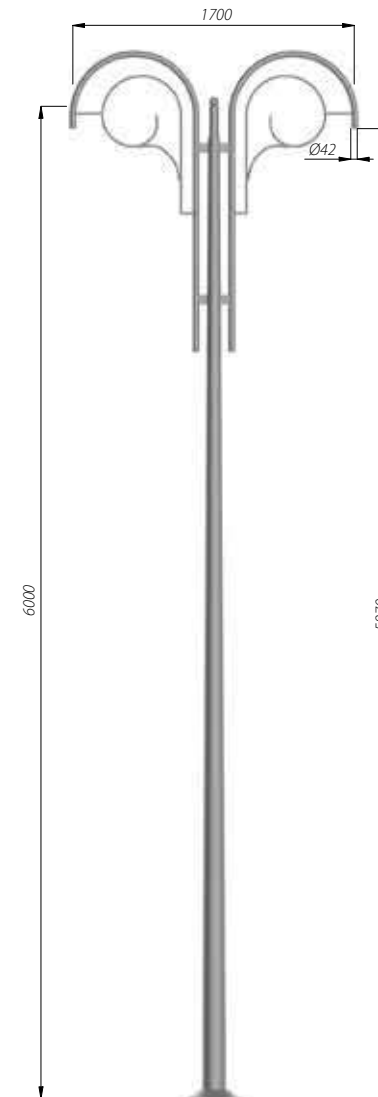
SAL-R2 code: 42311/C...
