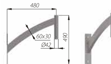
KA-C1 code: 478102/C... luminarias: OW LED, DROP LED, OW
