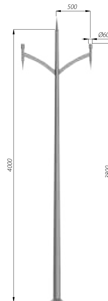
SAL-D1 code: 42215/C...
