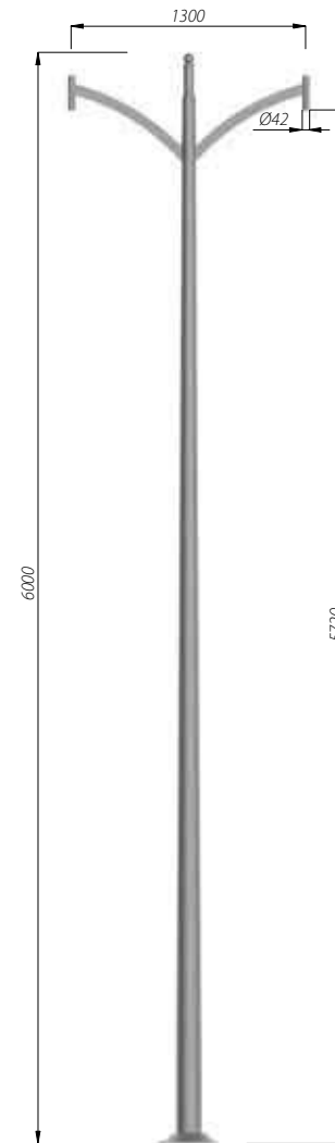
SAL-K2 code: 42306/C...
