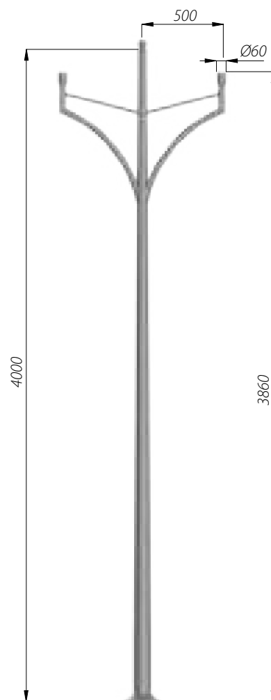
SAL-A2 code: 42210/C..
