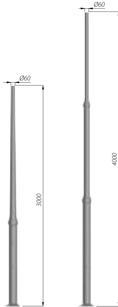
SAL DP-31 code: 42910/C...
